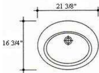
Space saver w/water rim
